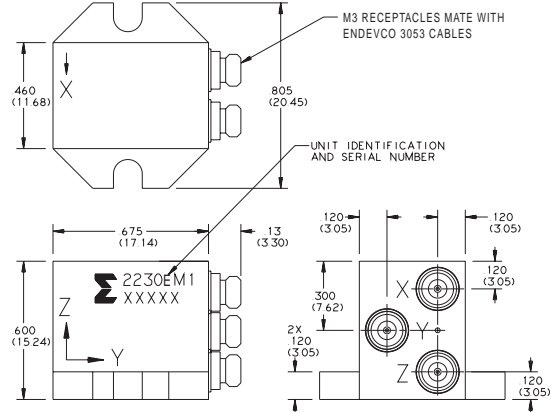
OUTLINE DRAWING
