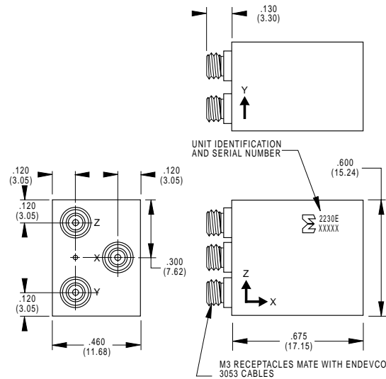
OUTLINE DRAWING
